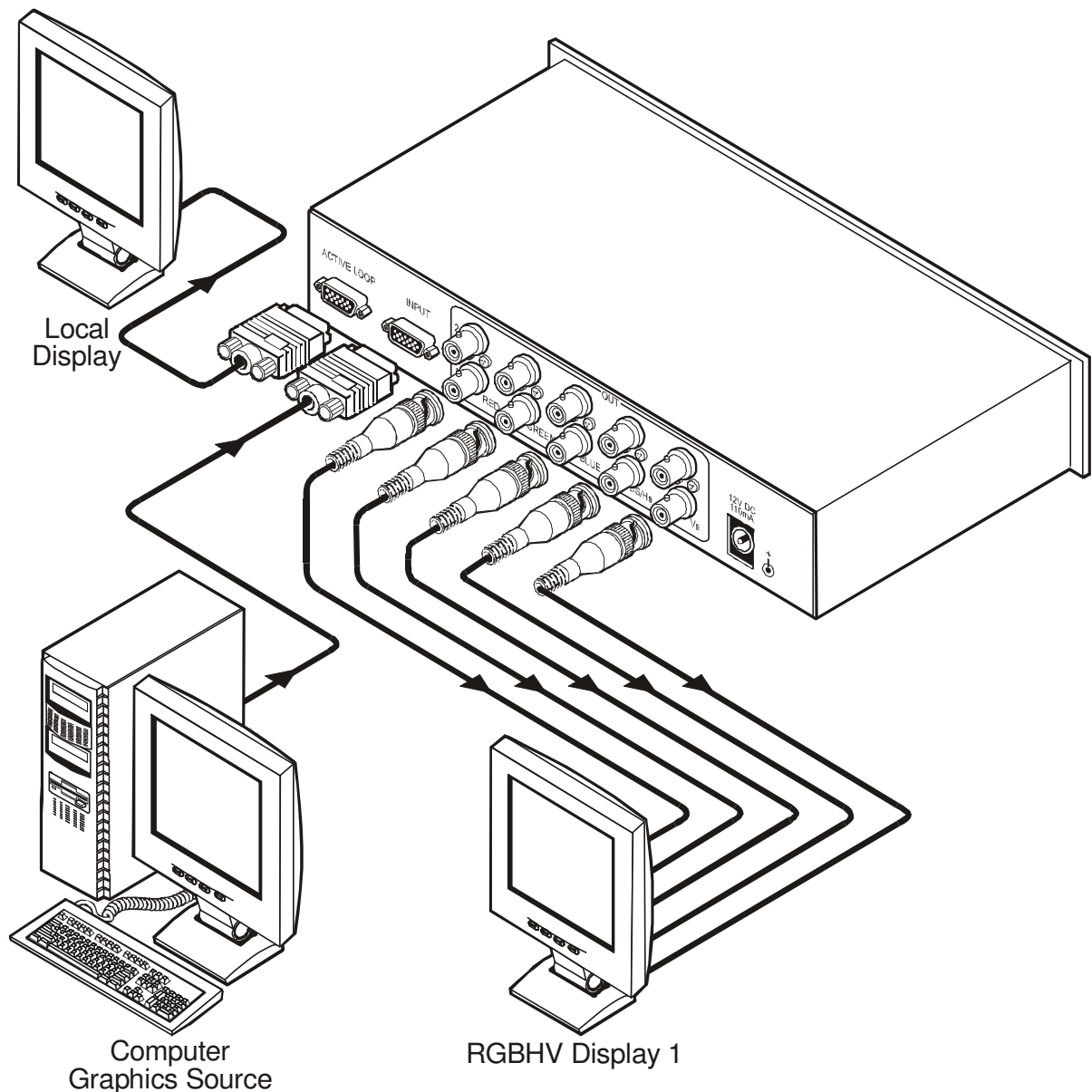
Figure 2: Connecting the VP-103 XGA Line Amp/Converter
