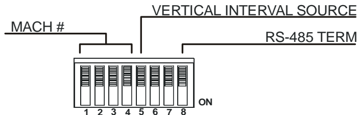
Figure 9: DIP-switch Settings
