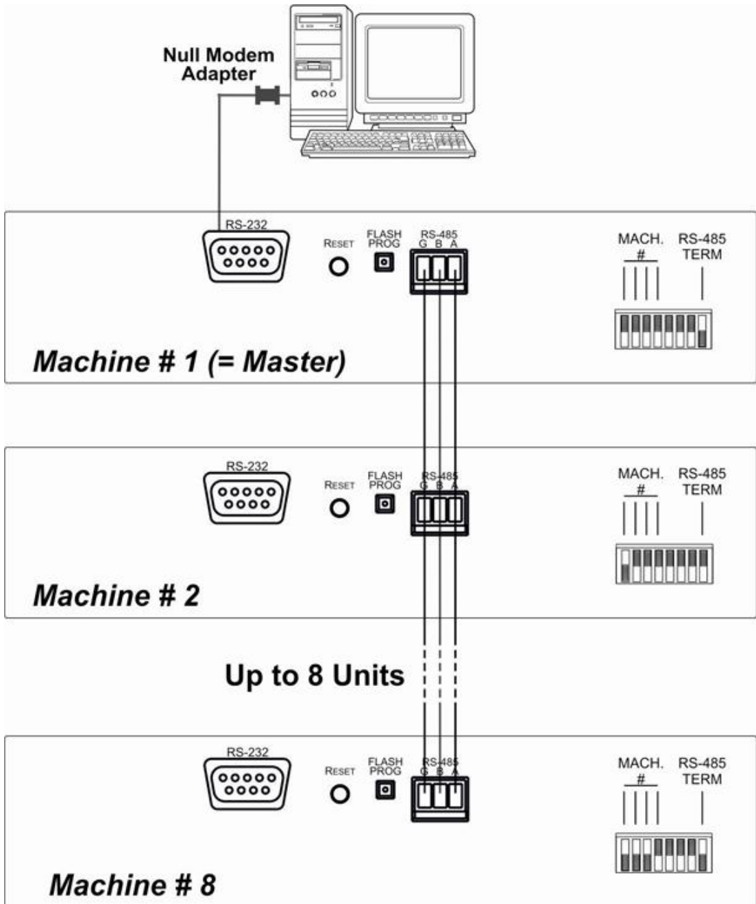
Figure 10: Cascade Configuration for RS-232/RS-485 Control
