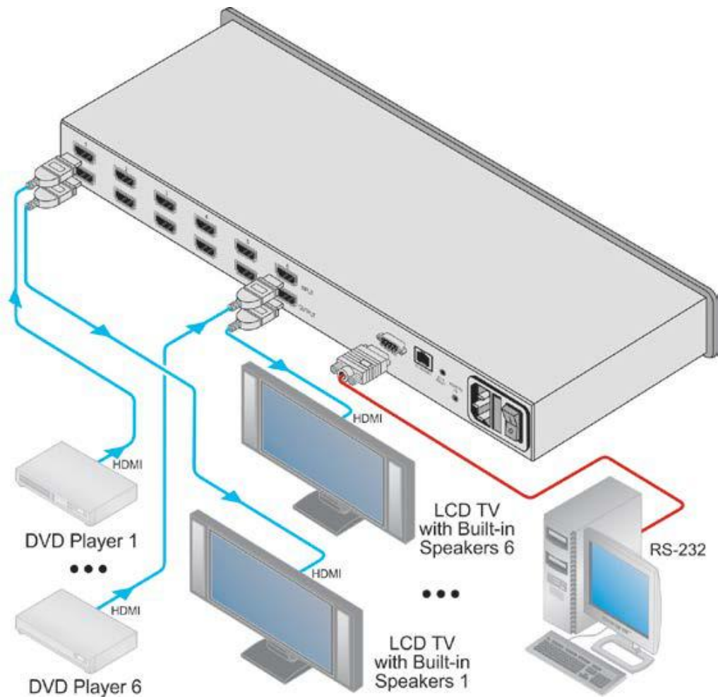
Figure 3: Connecting the VS-66HN 6x6 HDMI Matrix Switcher
