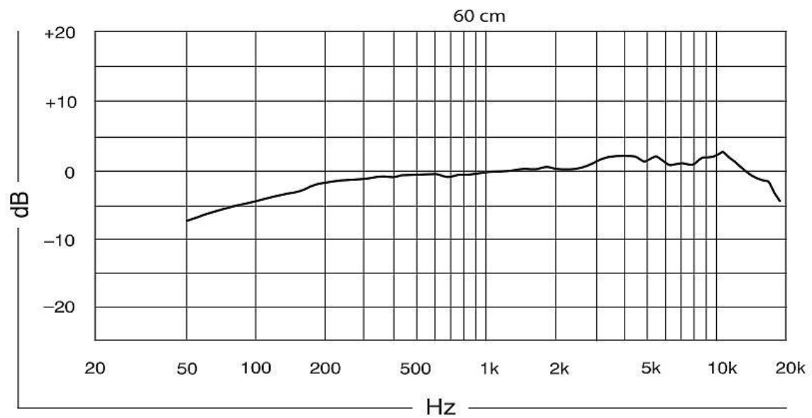
Frequency Response
