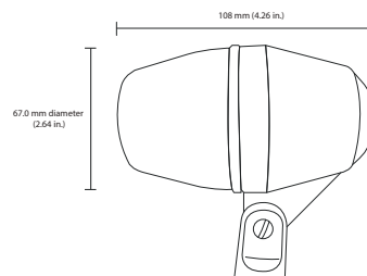
Overall Dimensions
