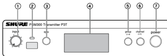
P3T Front Panel
