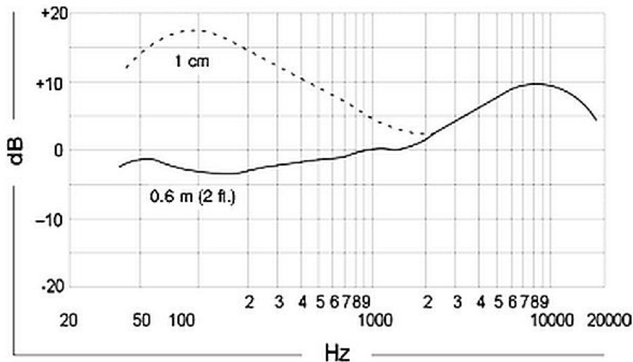
TYPICAL FREQUENCY RESPONSE
