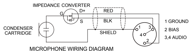
MICROPHONE WIRING DIAGRAM
