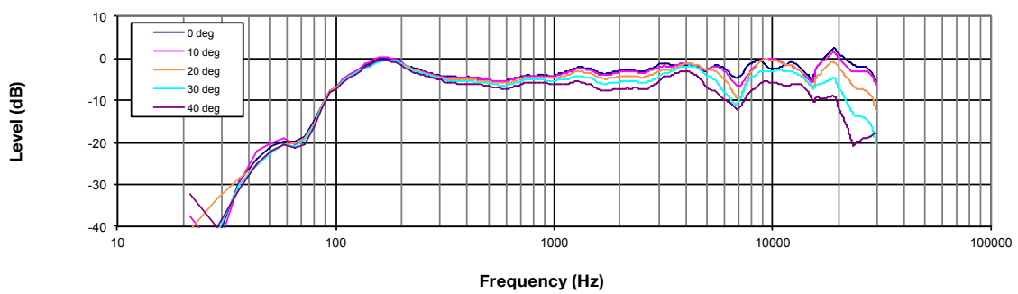
Off-axis Frequency Response
