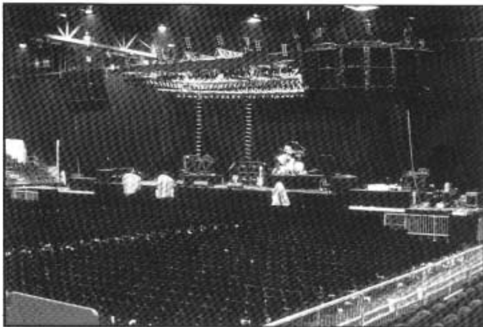
Turbosound TMS-3 enclosures and FB-300 flying bars in use at the National Exhibition Centre, Birmingham, U.K.
